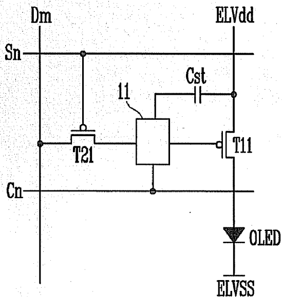
FIG. 2 (RELATED ART)
