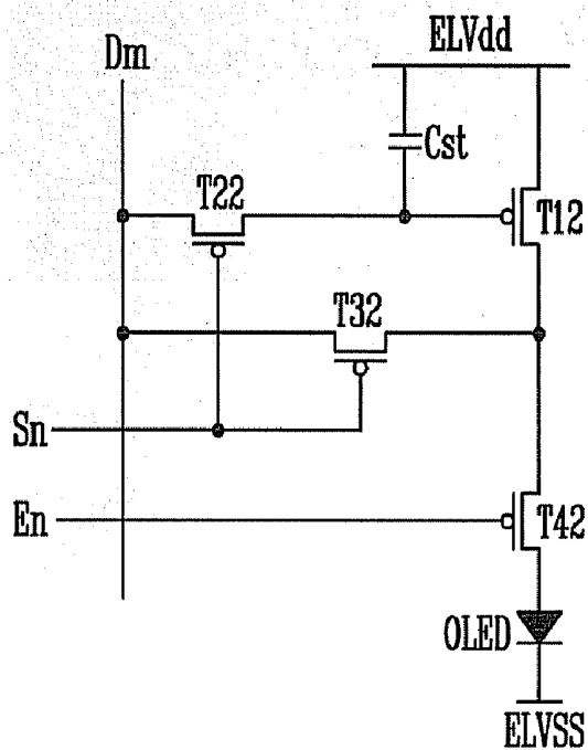
FIG. 2 (RELATED ART)
